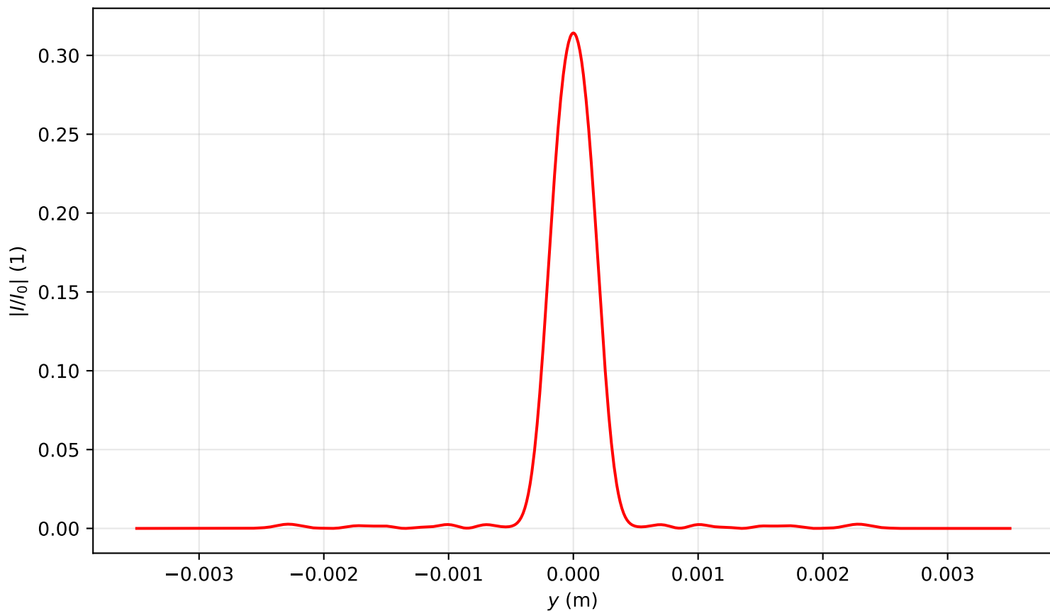
Intensity profile I(x=0, y, z=3.503)/I_0 , P_{in}=7.0P_{cr} , artificial time
